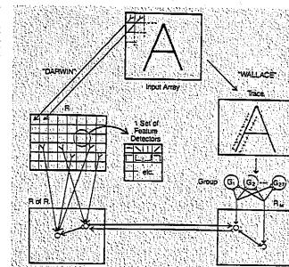
Figure 2. Simplified construction plan for Darwin II.
