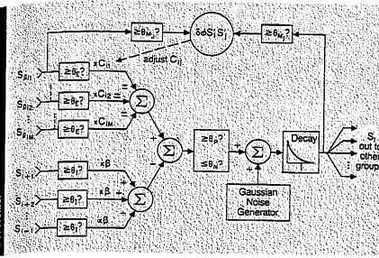
Figure 1. Logical structure of a group in Darwin II. All the repertoires in the automaton are made by connecting together groups that have a common logical structure, as summarized in Figure 2.
